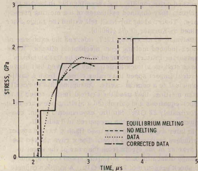
FIG. 37. Calculated and experimentally observed wave profiles for bismuth shock loaded at 2.1 GPa, at an initial temperature of 493 K. After Johnson et al. (1974).
