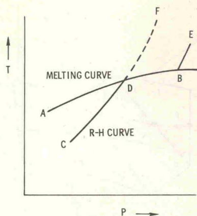
FIG. 33. Temperature-pressure phase diagram and R-H curve.
